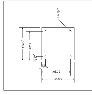
MOUNTING PLATE DETAIL
