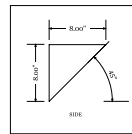
BRACKET DETAIL
