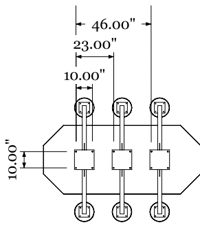
MOUNTING PLATE PATTERN DIMENSIONS
