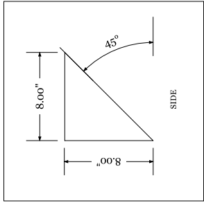
BRACKET DETAIL
