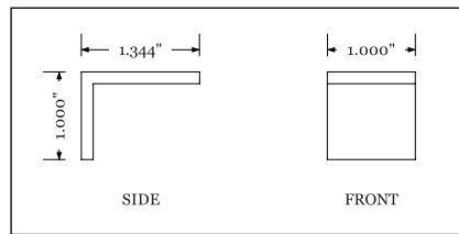
DETAIL OF LADDER HOOK
