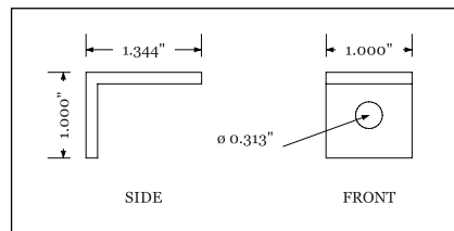
DETAIL OF LADDER BRACE
