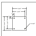
MOUNTING PLATE DETAIL
