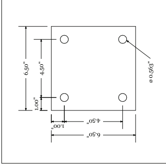
FLOOR MOUNT DETAIL
