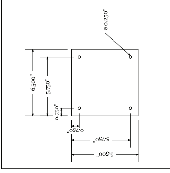
MOUNTING PLATE DETAIL
