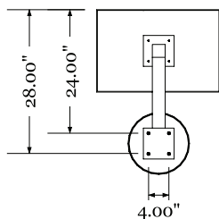
MOUNTING HOLE PATTERN DIMENSION
